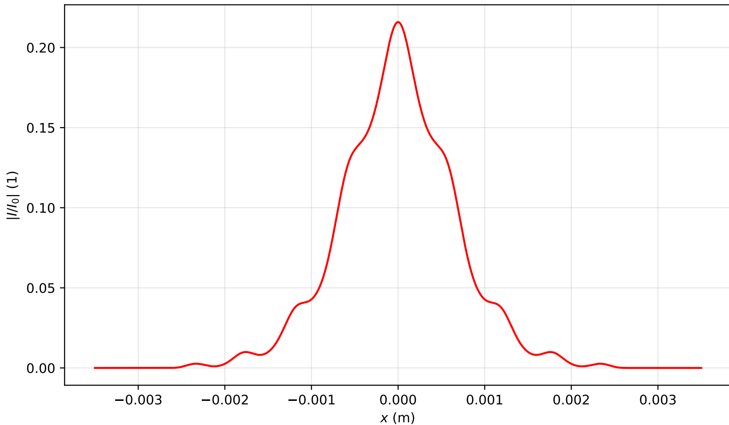
Intensity profile I(x, y = 0, z = 3.981)/I_0 , P_{in}=1.0P_{cr} , artificial time
